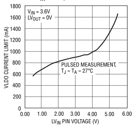
VLDO Current Limit vs V_{IN} Voltage
